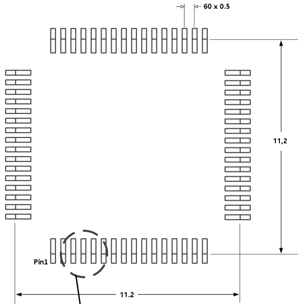
Example Board Layout
